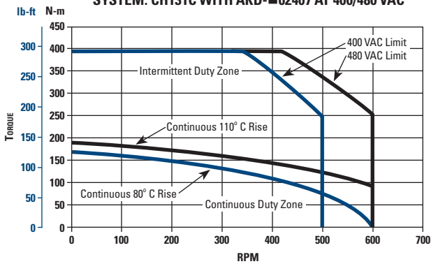
SYSTEM: CH133C WITH AKD-02407 AT 400/480 VAC
