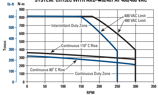
SYSTEM: CH132C WITH AKD-02407 AT 400/480 VAC
