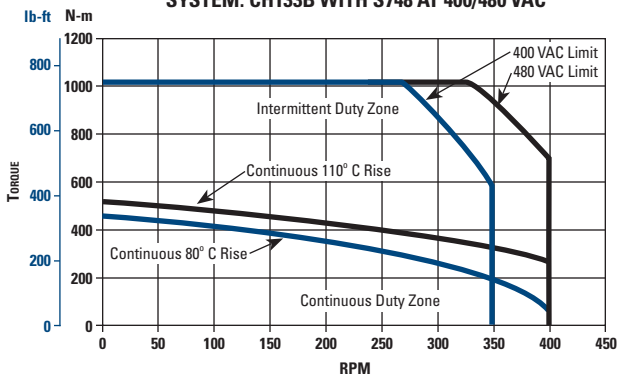
SYSTEM: CH133B WITH S748 AT 400/480 VAC
