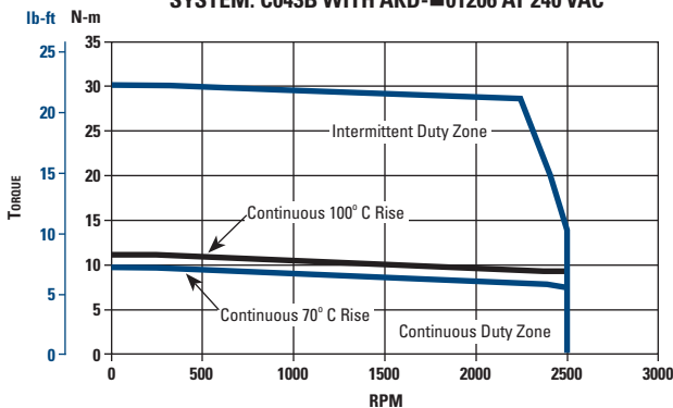
SYSTEM: C043B WITH AKD-01206 AT 240 VAC
