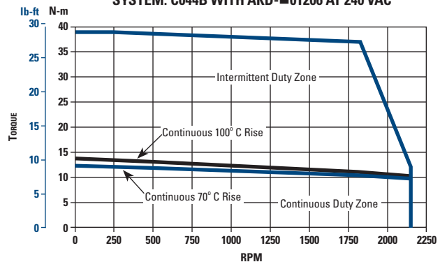
SYSTEM: C044B WITH AKD-01206 AT 240 VAC
